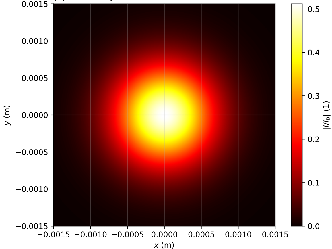
Intensity profile I(x, y, z = 2.866m)/I_0 , Pin=0.4Pcr, artificial time
